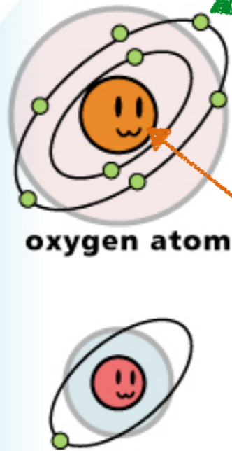
hydrogen atom
